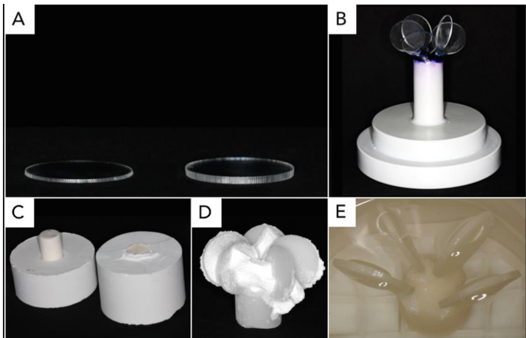
Fig. 1: Plastic sheets with thicknesses of 0.5 mm and 1.0 mm and diameter of 15 mm (A). Plastic sheets were attached to a ring mold with sprue (B). Investment was removed with a carborundum disc (C). Remaining investment was sandblasted with aluminum oxide (D) and ultrasonically cleansed with IPS Invox Press liquid (E).
