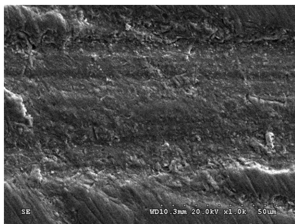
Fig. 5: Scanning electron micrograph of Er-YAG laser irradiated zirconia surface revealed roughness and scaly appearance without microcracks at \times 1,000 magnification
