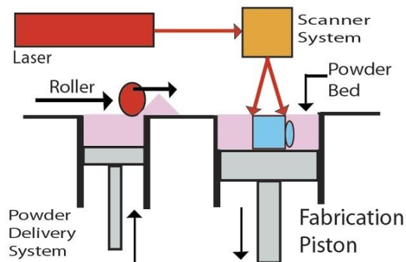
Fig. 3: Selective Laser Sintering
