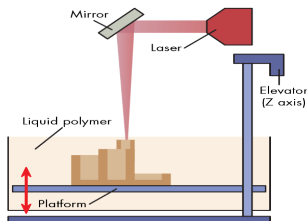
Fig. 1: Stereo Lithography
