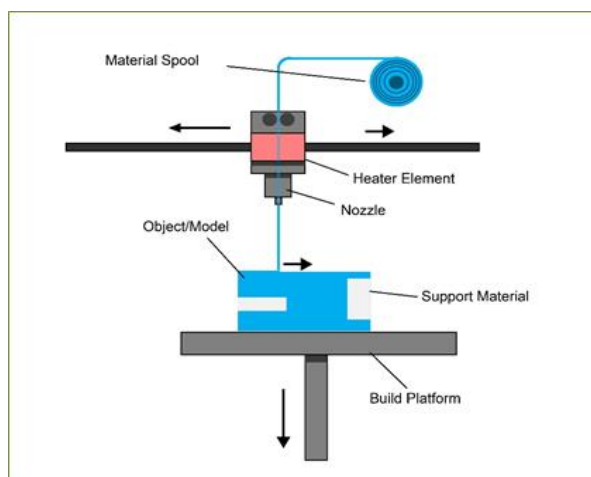
Fig. 2: Fused Deposition Modelling
