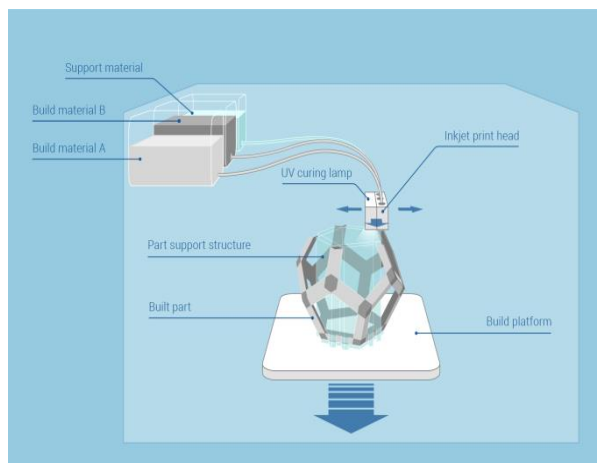
Fig. 4: Photopolymer Jetting
